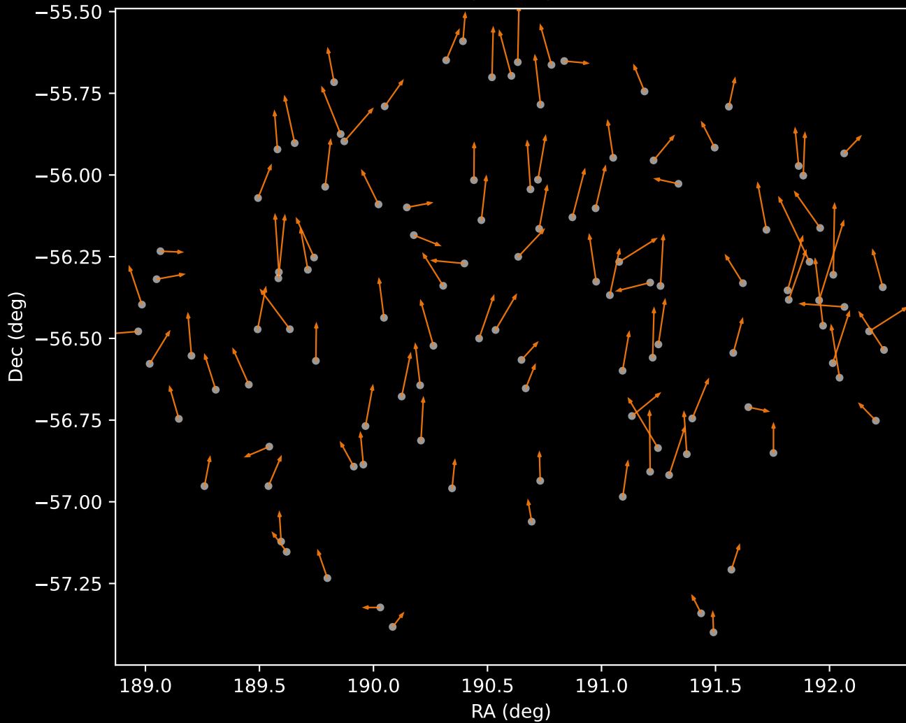
GALAH DR4 Cluster 2 Proper Motion Vectors (n=114)
