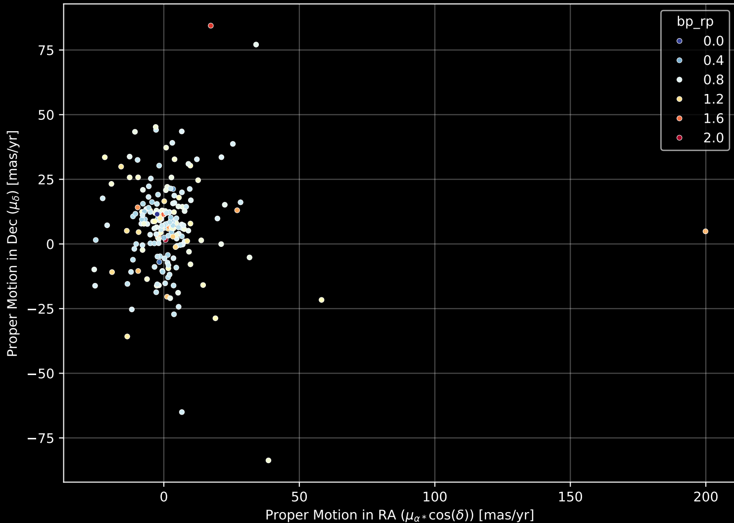
GALAH DR4 Field: [7187] Proper Motion Diagram (n= 198)
