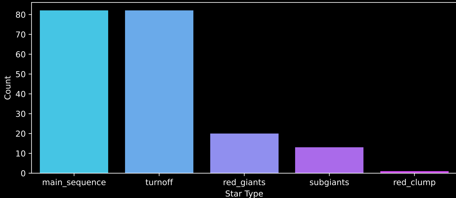
GALAH DR4 Field: [7187] Count plot of Star Type
