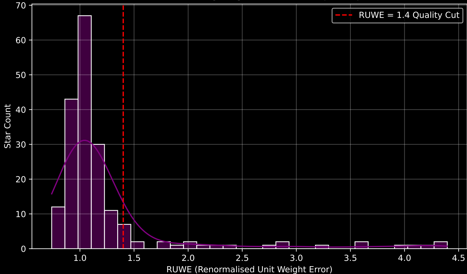
GALAH DR4 Field [7187] RUWE Distribution (n= 191)
